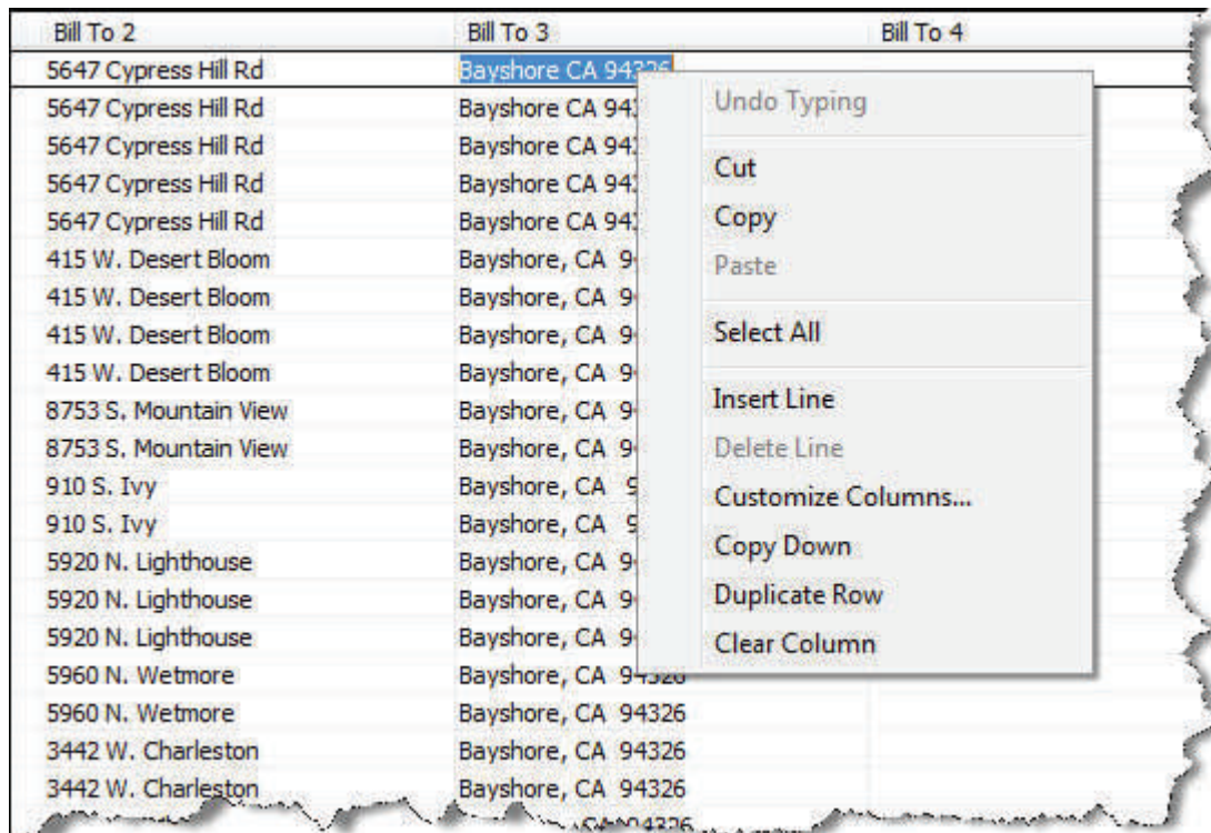
Figure 4: The Copy Down command changes all entries in a column to match the top one.
